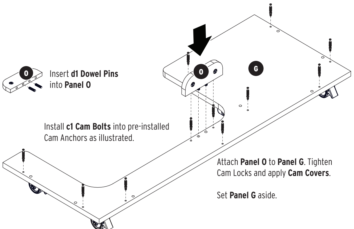
c2 \frac{5}{8} " Cam Cover x2
